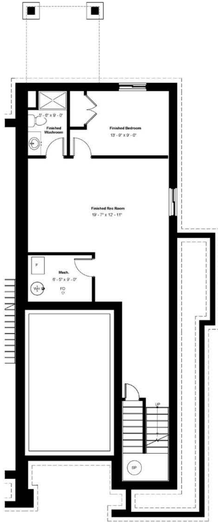
Basement
