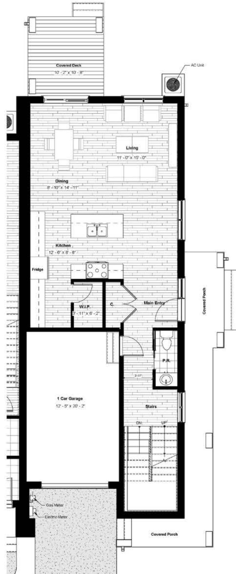
Main Floor 905 sq ft
