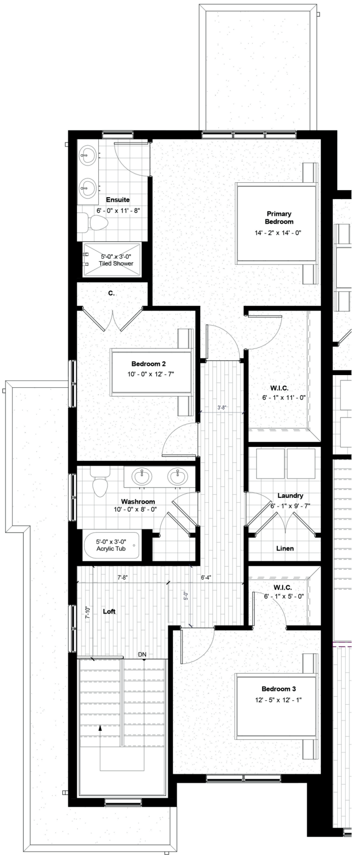
Second Floor 1100 sq ft
