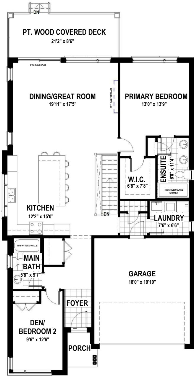
MAIN FLOOR - 1583 SQ.FT. - 9' CEILING
