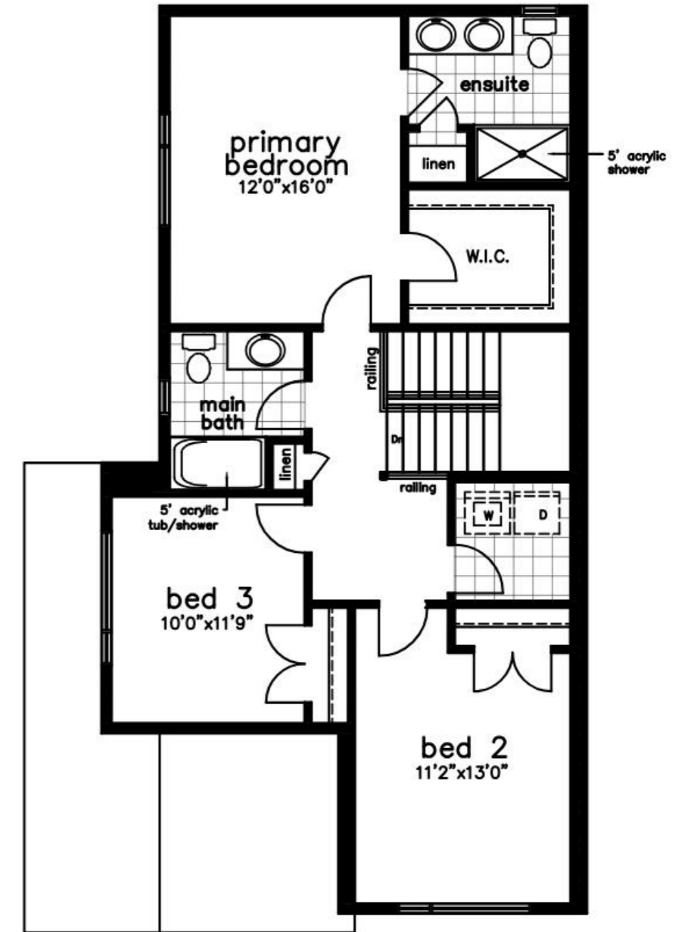
Second Floor - 962 sq ft 8' ceilings
