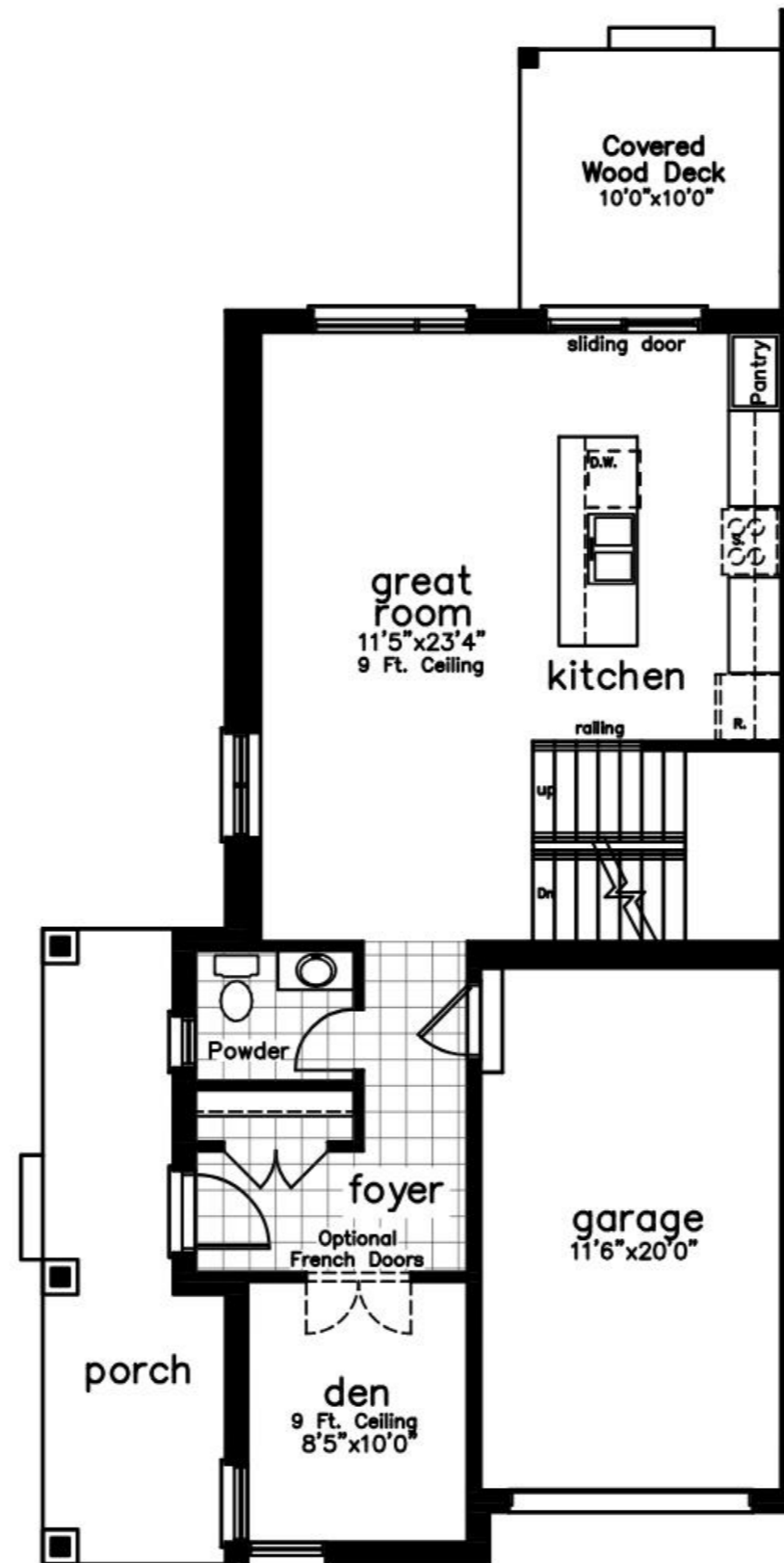
Main Floor - 800 sq ft 9' ceilings
