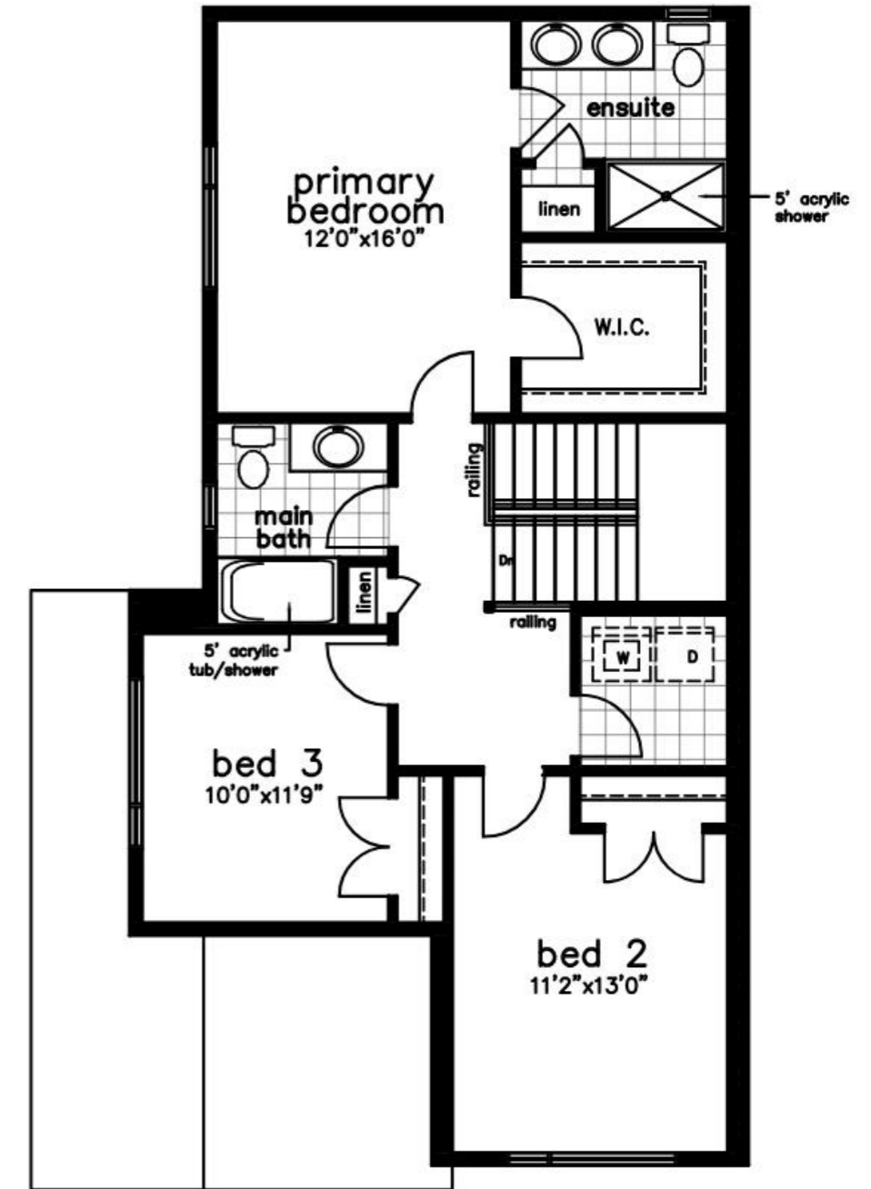
Second Floor - 973 sq ft 8' ceilings
