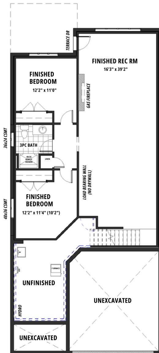
BASEMENT 1152 SQ FT [8'4" POUR]
