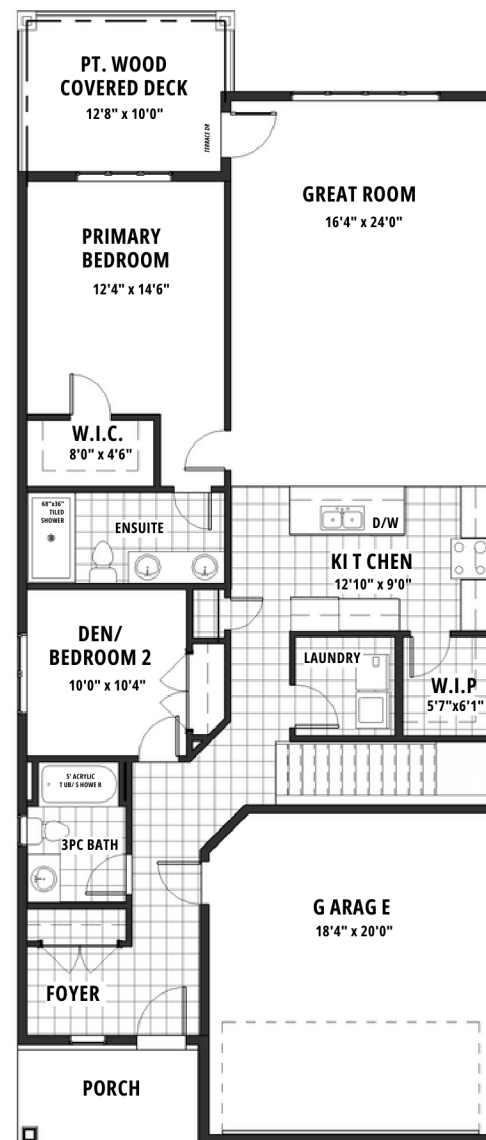
MAIN FLOOR 1462 SQ FT [9' CEILING]
