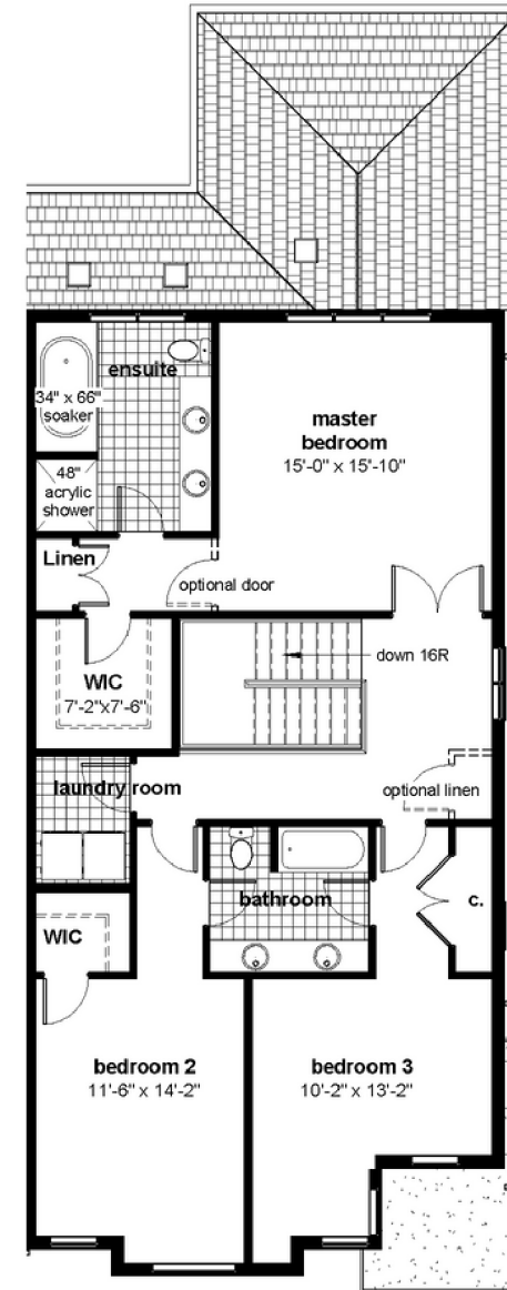
SECOND FLOOR 1366 SQ FT [8' CEILING]
