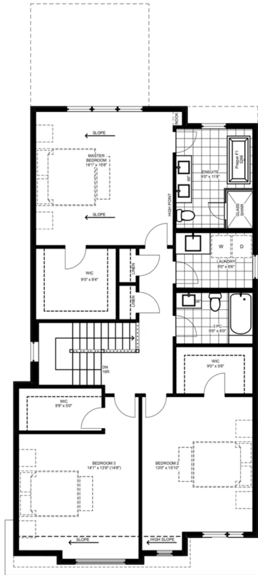
SECOND FLOOR 1412 SQ FT [8' CEILING]
