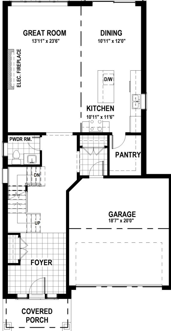
MAIN FLOOR - 1158 SQ.FT. - 9' CEILINGS
