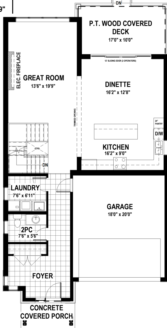
MAIN FLOOR - 1197 SQ.FT. - 9' CEILINGS
