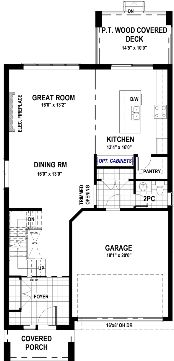
MAIN FLOOR - 1164 SQ.FT. - 9' CEILINGS
