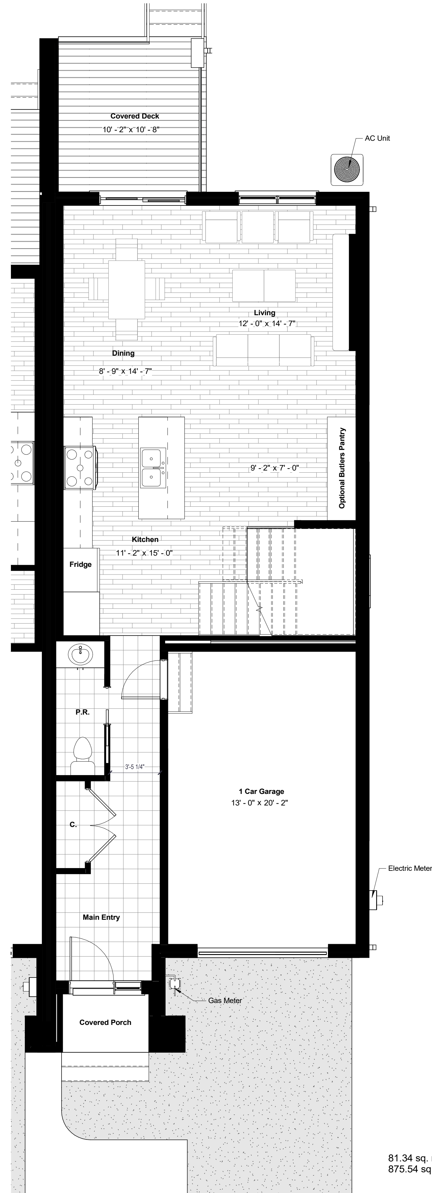
2 Enlarged Plan - Unit Type A - First Floor Level M4001 scale: 1/4" = 1'-0"
