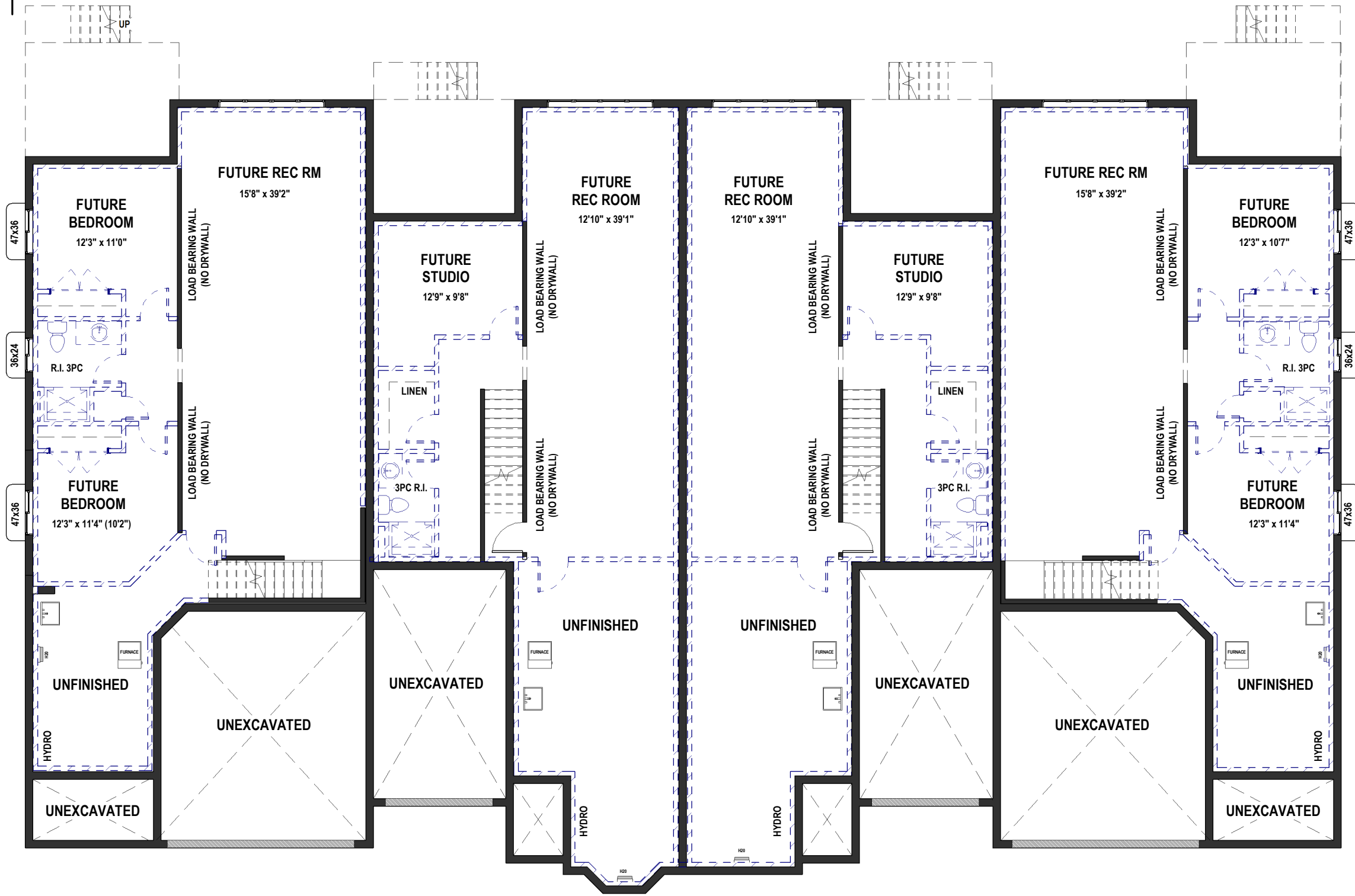
UNIT 24 TYPE - C
