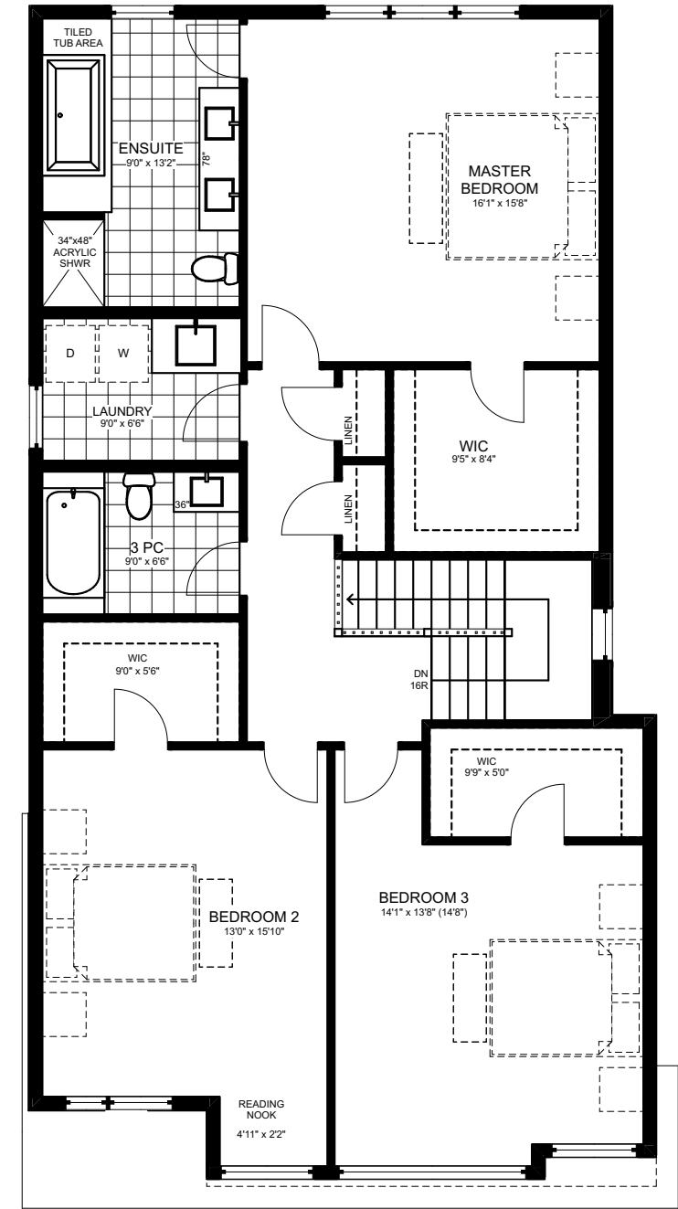
SECOND FLOOR - 8' CEILINGS 1,440.7 sq ft
