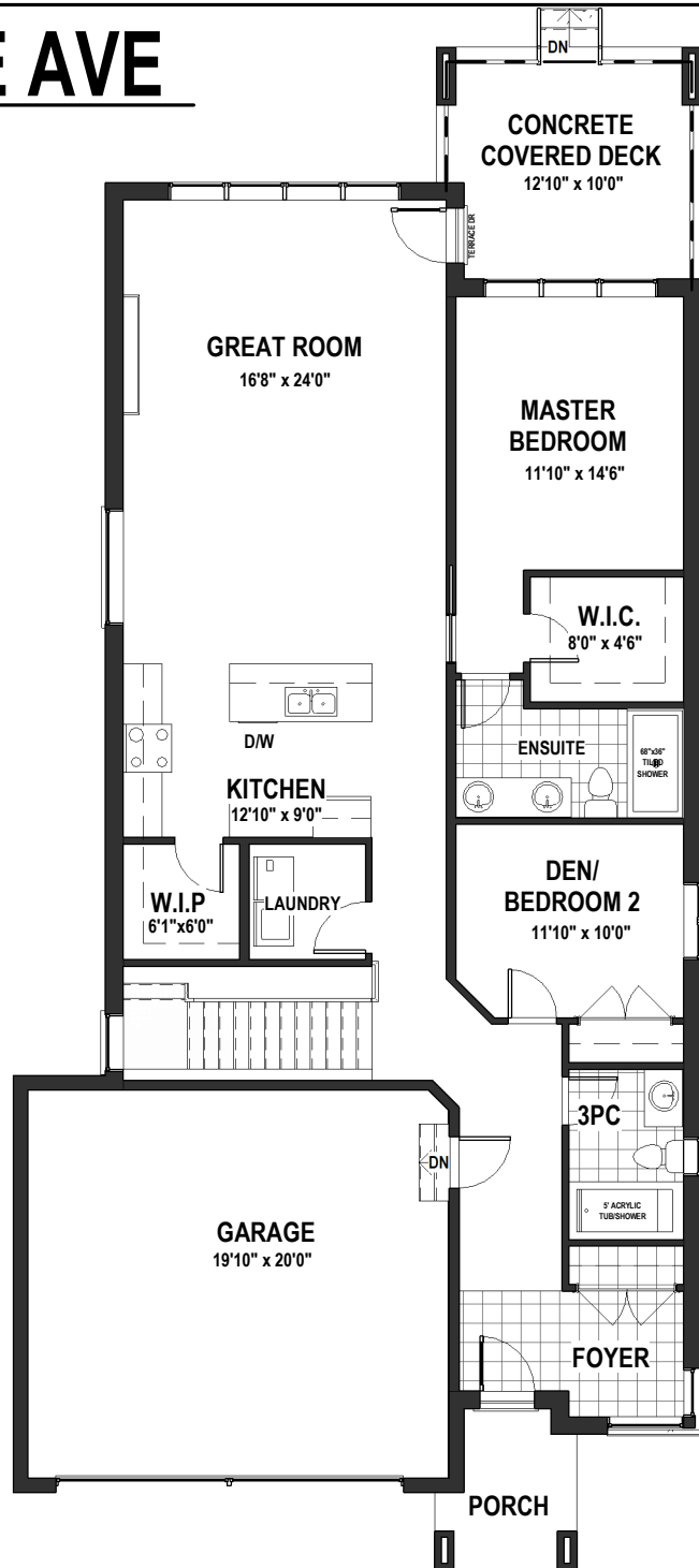
MAIN FLOOR - 1614 SQ.FT - 9' CEILINGS
