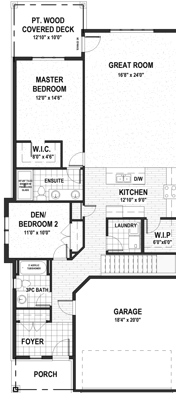
MAIN FLOOR TYPE - C4 1480 SQ.FT. - 9' CEILINGS
