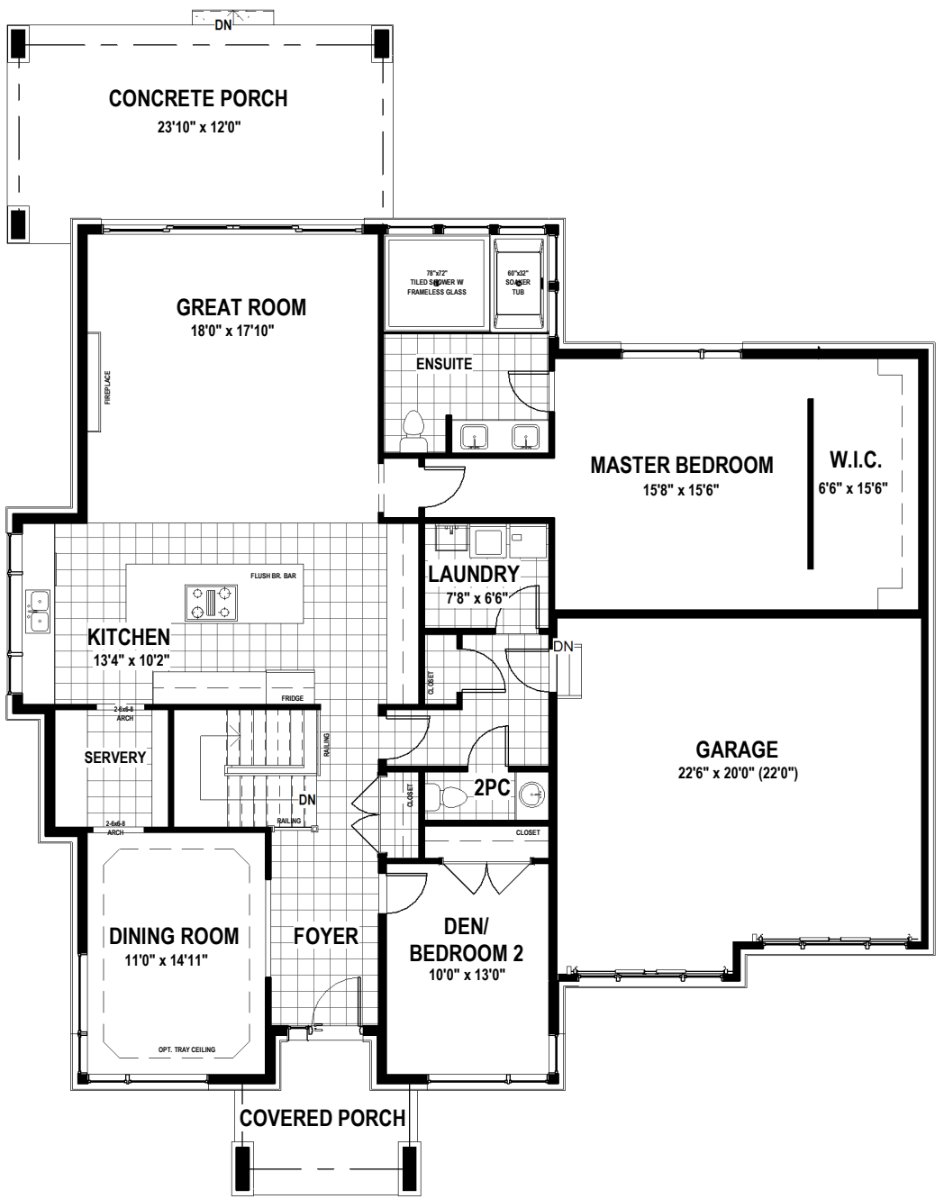
MAIN FLOOR - 2055 SQ.FT. - 9' CEILINGS
