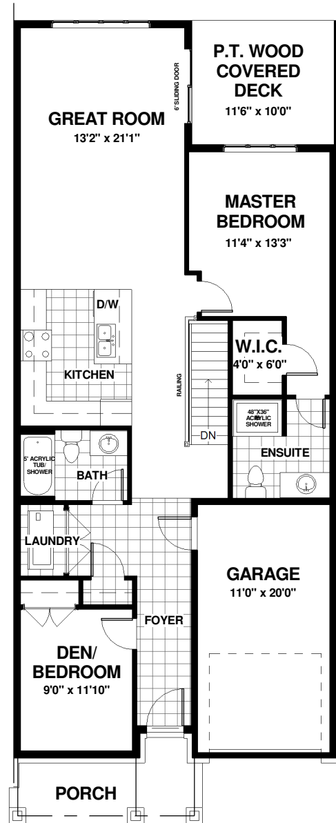
MAIN FLOOR - 1197 SQ.FT. TYPE - E
